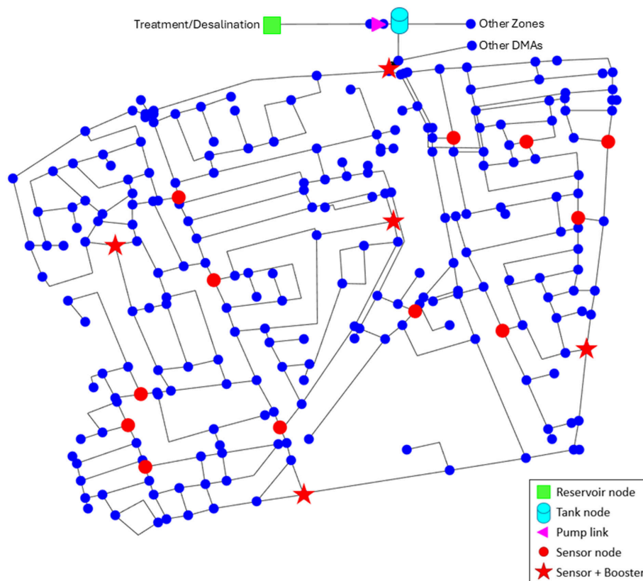
Fig. 2. CY-DBP network, containing one reservoir, one tank, 256 demand nodes, and 335 pipes, together with the location of the five chlorine booster stations, two flow sensors, and 17 chlorine sensors.
